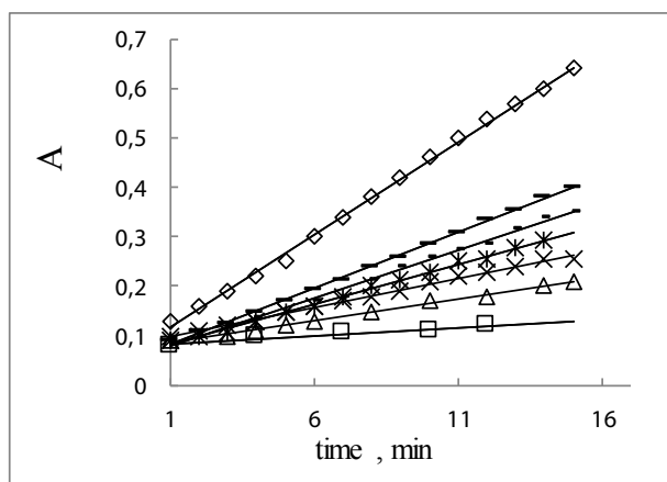
Fig. 2. Kinetic curves of couple oxidation of p -phenetidine by hydrogen peroxide in the system: 1 - ACh+ChE, 2- 6 - ACh+(ChE+BAC), 7 - ACh. w(\text{ACh}) = 0.1\% ; [\text{ChE}] = 0.25 \text{ U} ; c(\text{BAC}), 10^{-6} \text{ M} : 2-1.4, 3- 2.8, 4-3.4, 5 -5.6 , 6 - 7.0.
